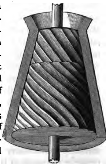
WINLAW'S MILL.
